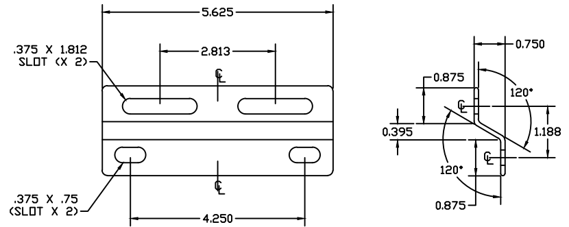
End View
