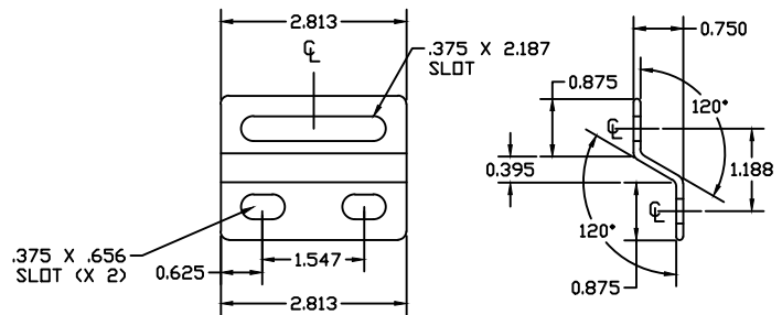
End View
